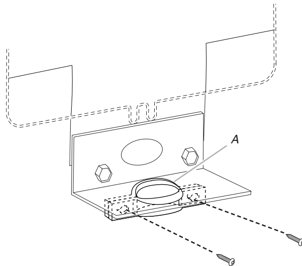
A. UL Listed strain relief
